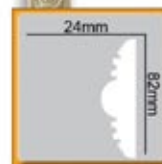
LR 3601 ER: 650mm IR: 568mm L1: 895mm L2: 1023mm
