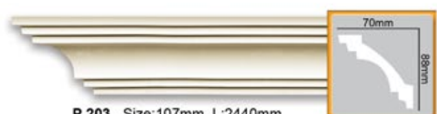
P 203 Size:107mm L:2440mm
